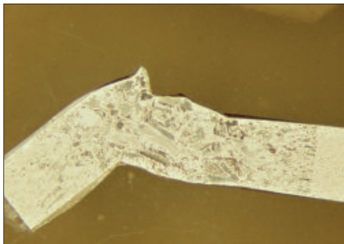
Fig. 10. Rough grain structure in the heat affected zone of plasma
